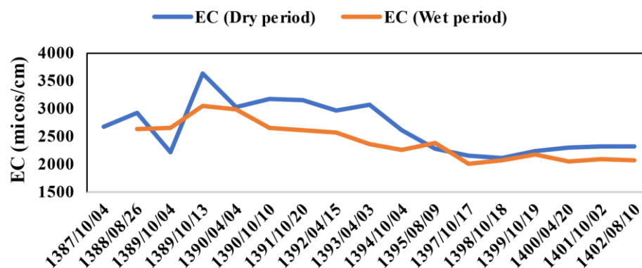
Figure 1- Temporal variation of EC in dry and wet period in case study
