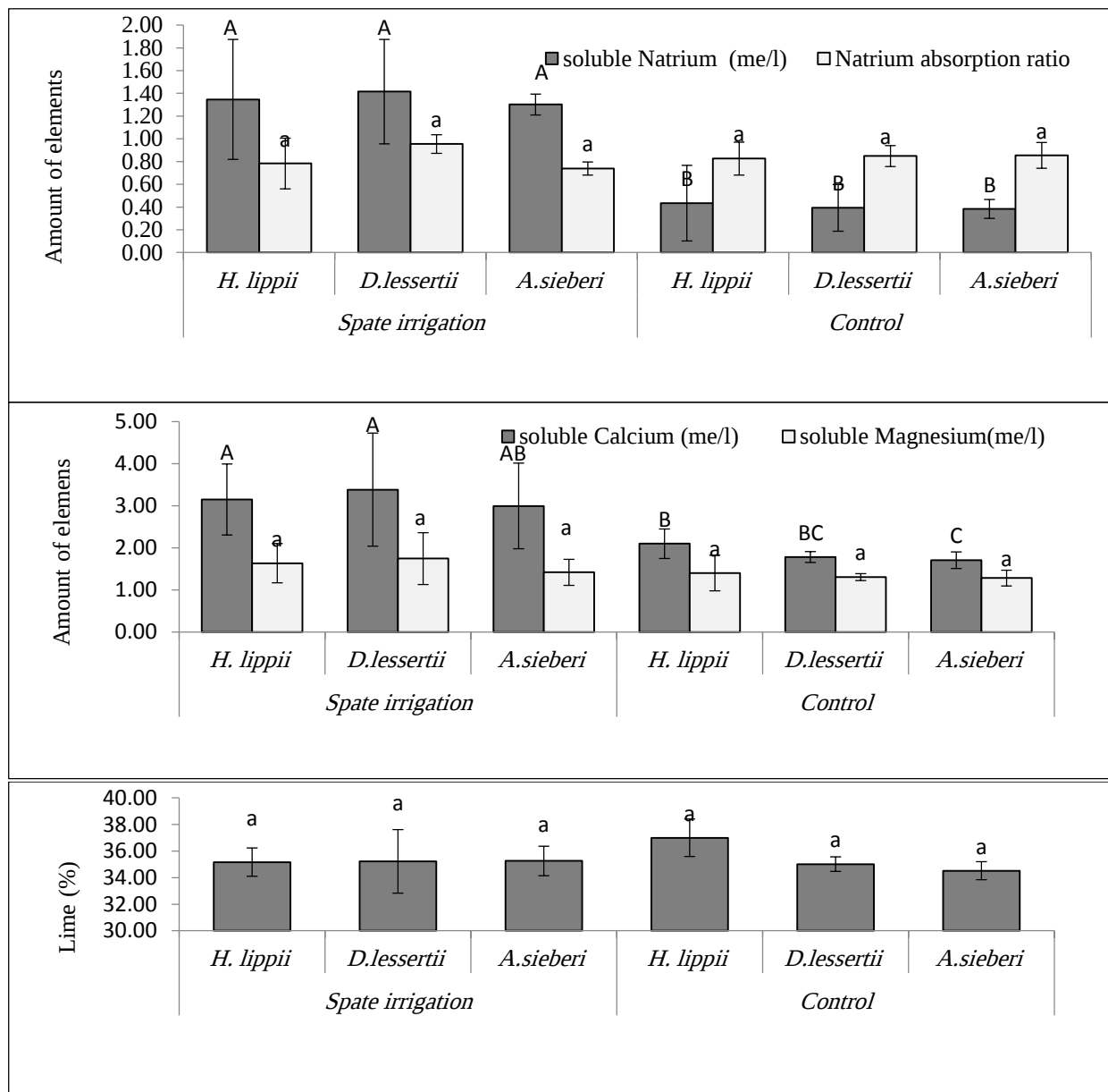
Figure 4- Soil elements of different types in flood spreading and non-flooding lands (control)
