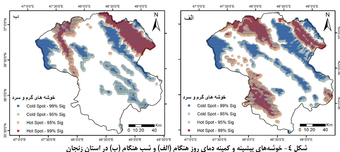
Figure 4- The maximum and minimum clusters of day (الف) and night (ب) temperatures in Zanjan Province
